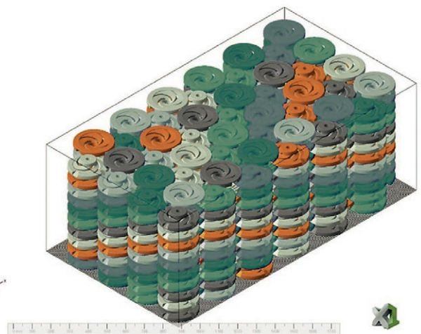
Figure 1 Up to 480 impeller cores can be printed in one jobbox per printing process. The illustration shows the ideal arrangement of the workpieces.
